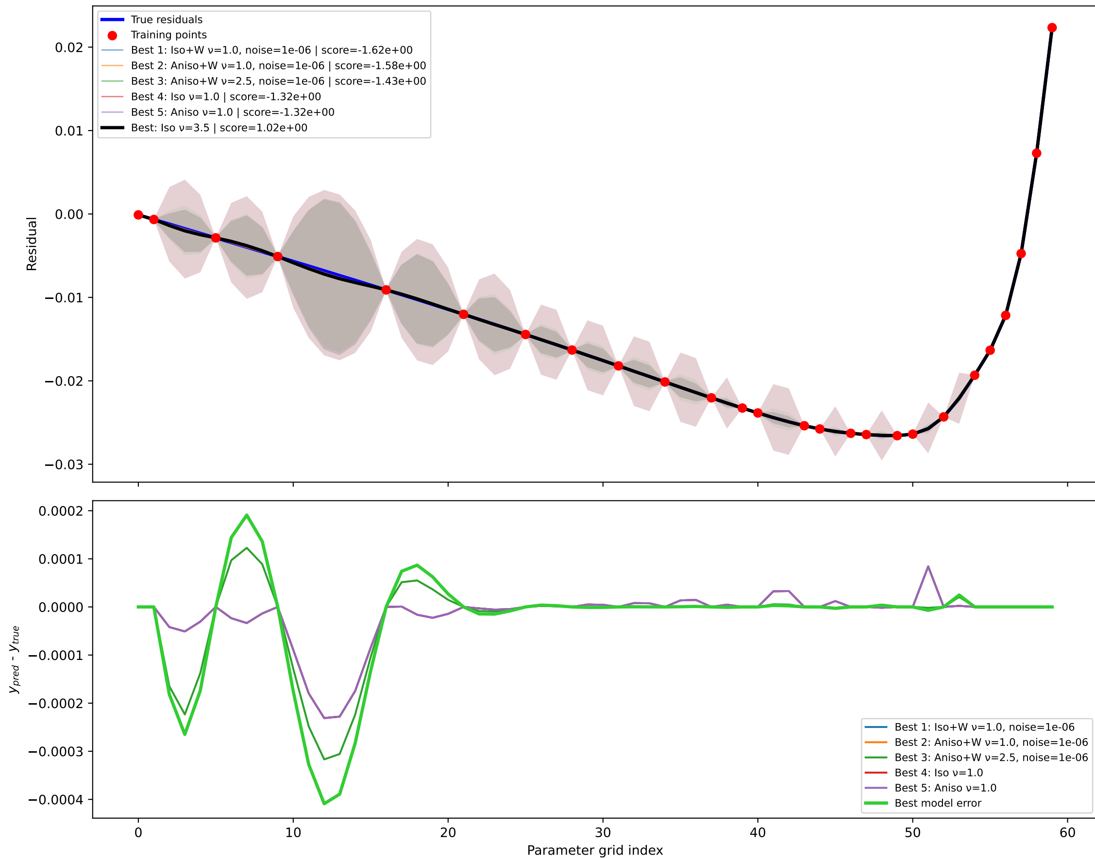
GPR kernel comparison node=0 RMSE=1.142e-04, train RMSE=1.448e-11
